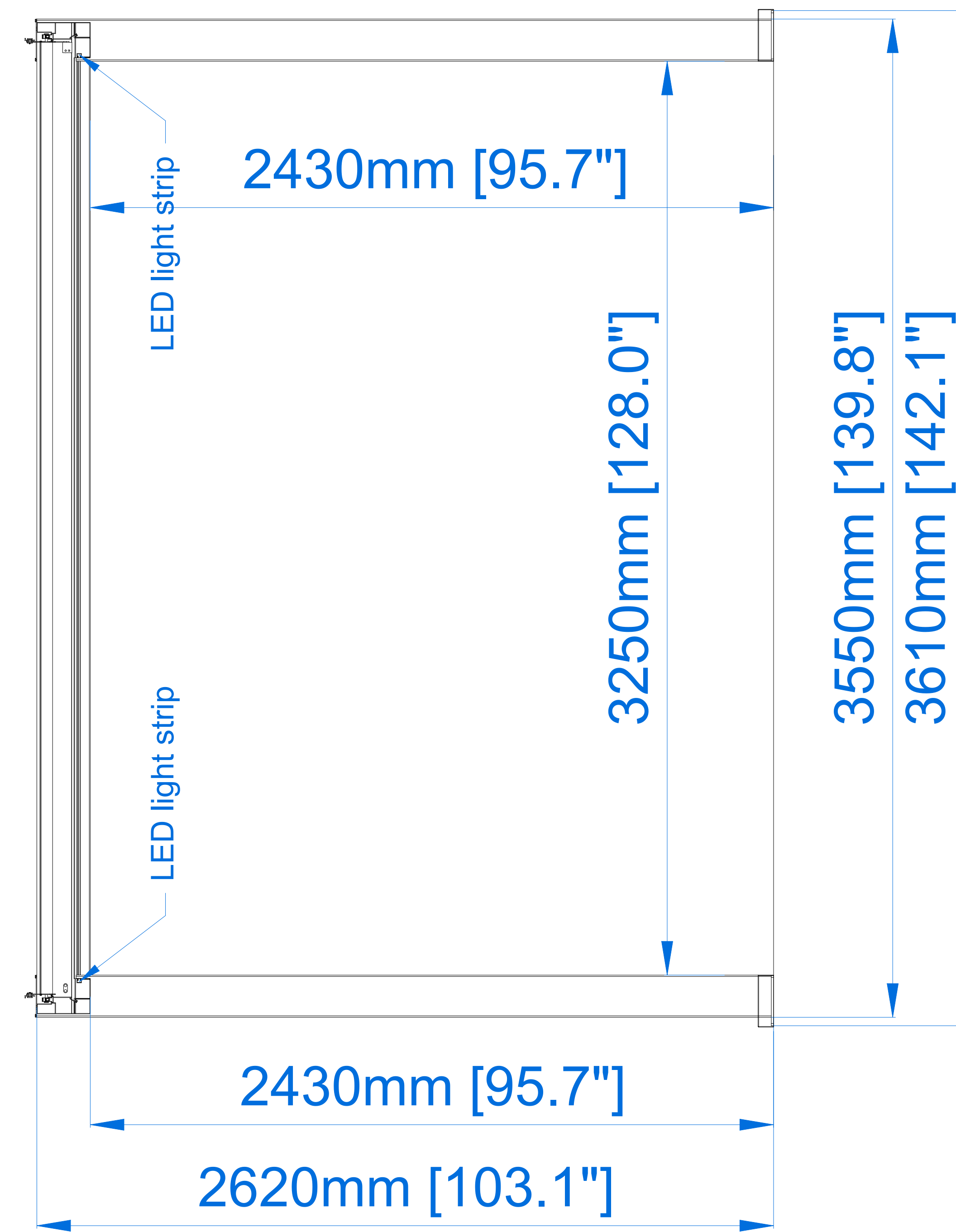
ELEVATION VIEW
