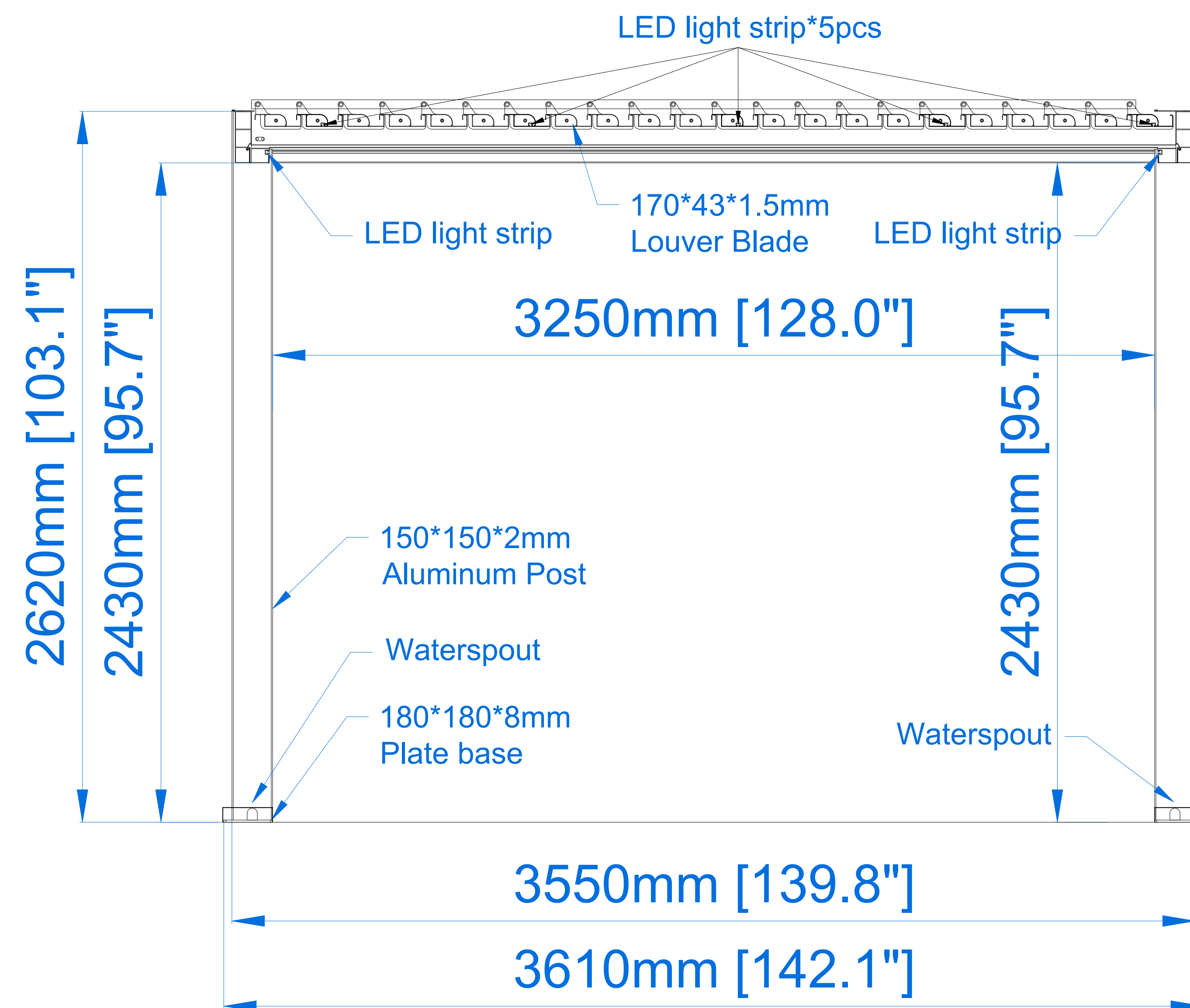
ELEVATION VIEW
