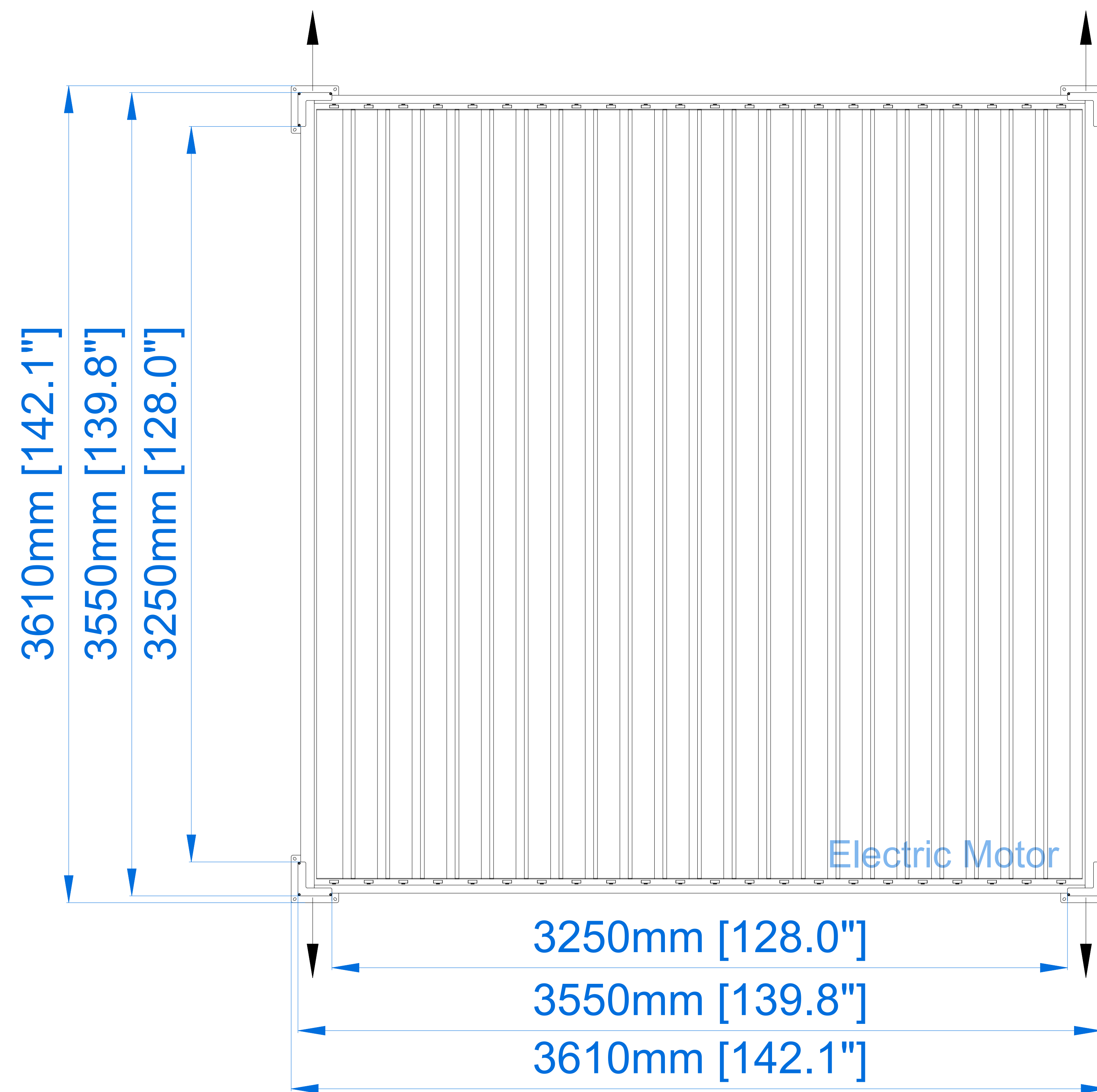
PLAN VIEW
